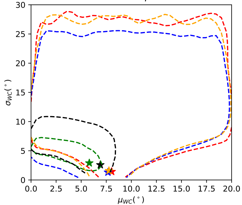
Hot Classical \mu and \sigma
