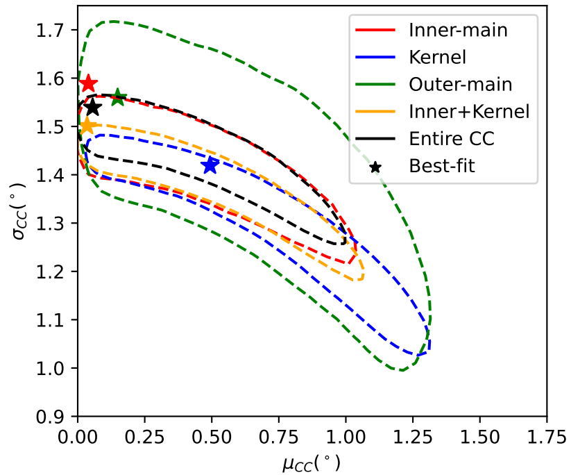
Cold Classical \mu and \sigma
