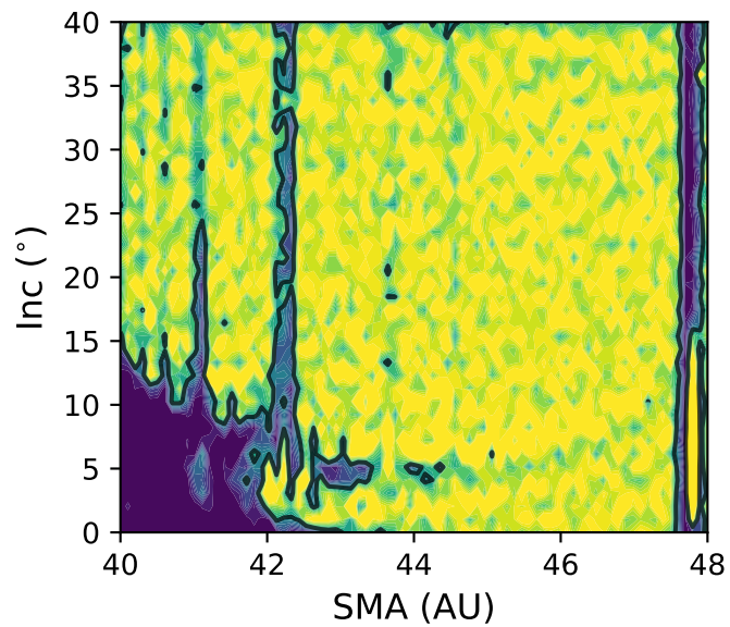
Density Ratio: e_{init} < 0.1 TNOs
