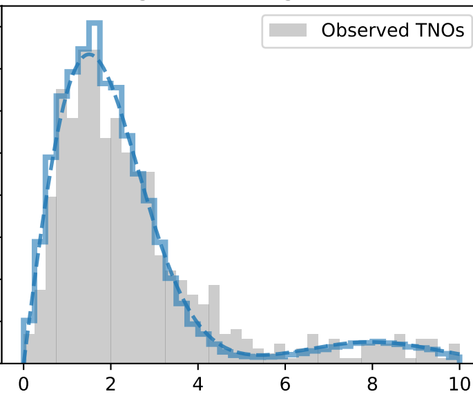
Surviving Osculating Inclinations
