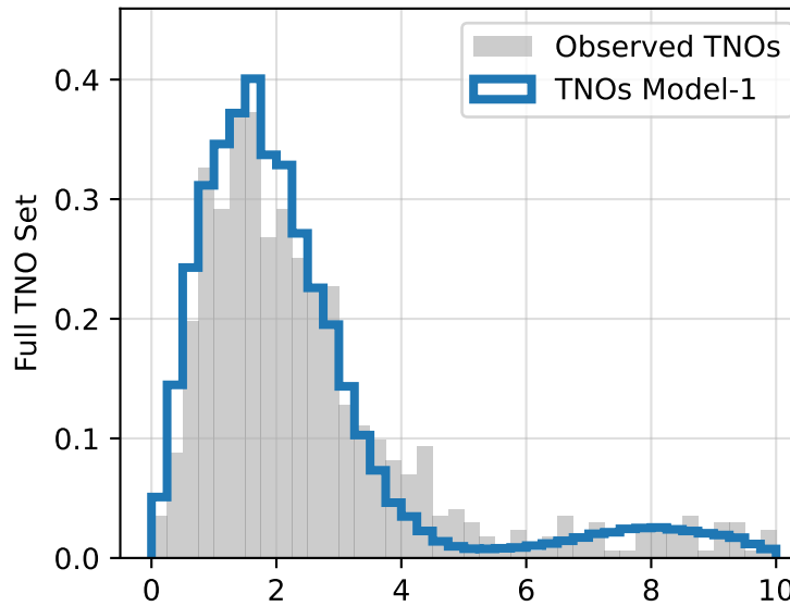
Inclination ( ^{\circ} )
