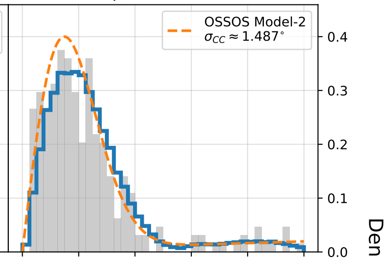
Proper Inclination
