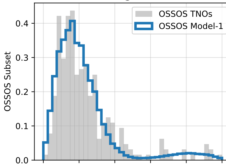
Osculating Inclination
