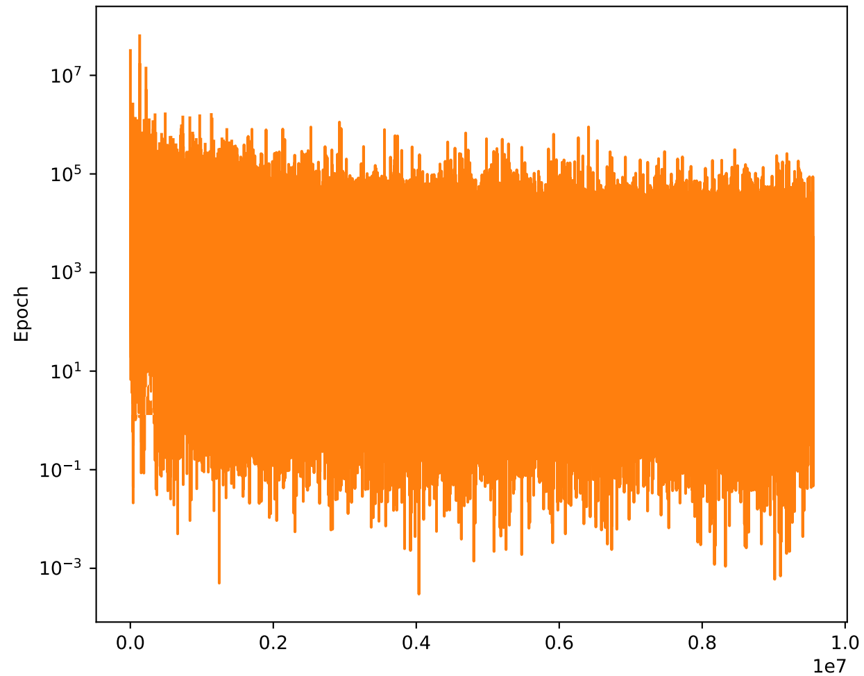
Critic Loss
