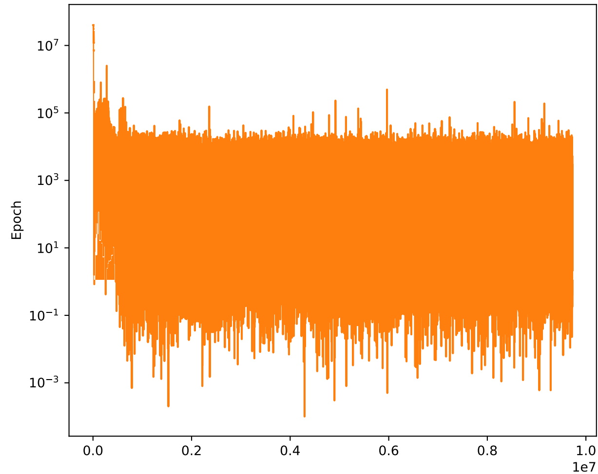
Critic Loss
