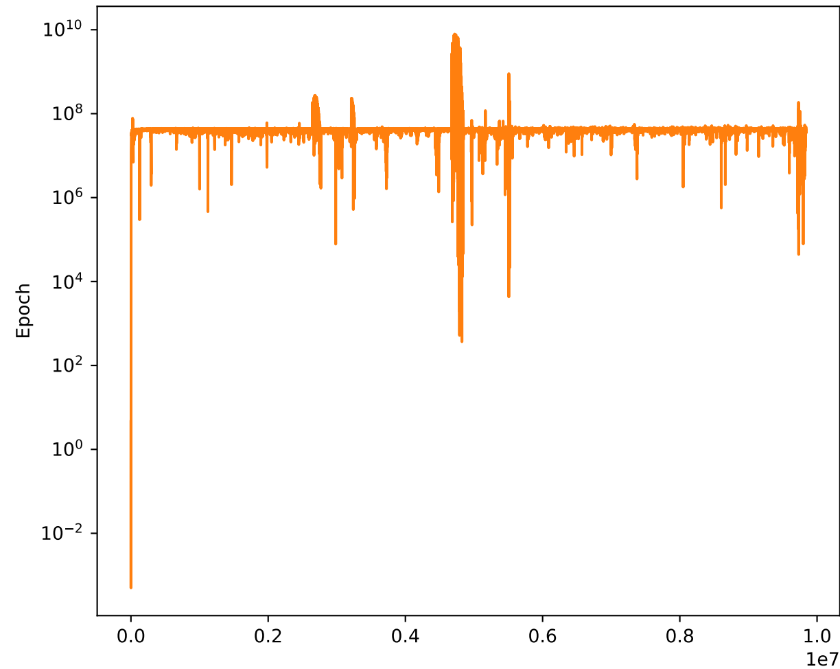
Critic Loss
