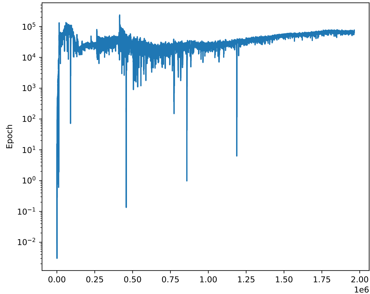
Generator Loss
