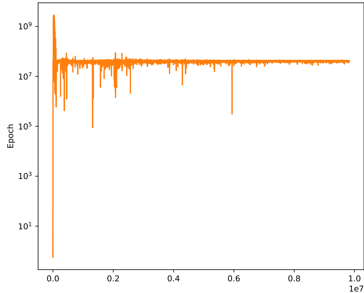
Critic Loss
