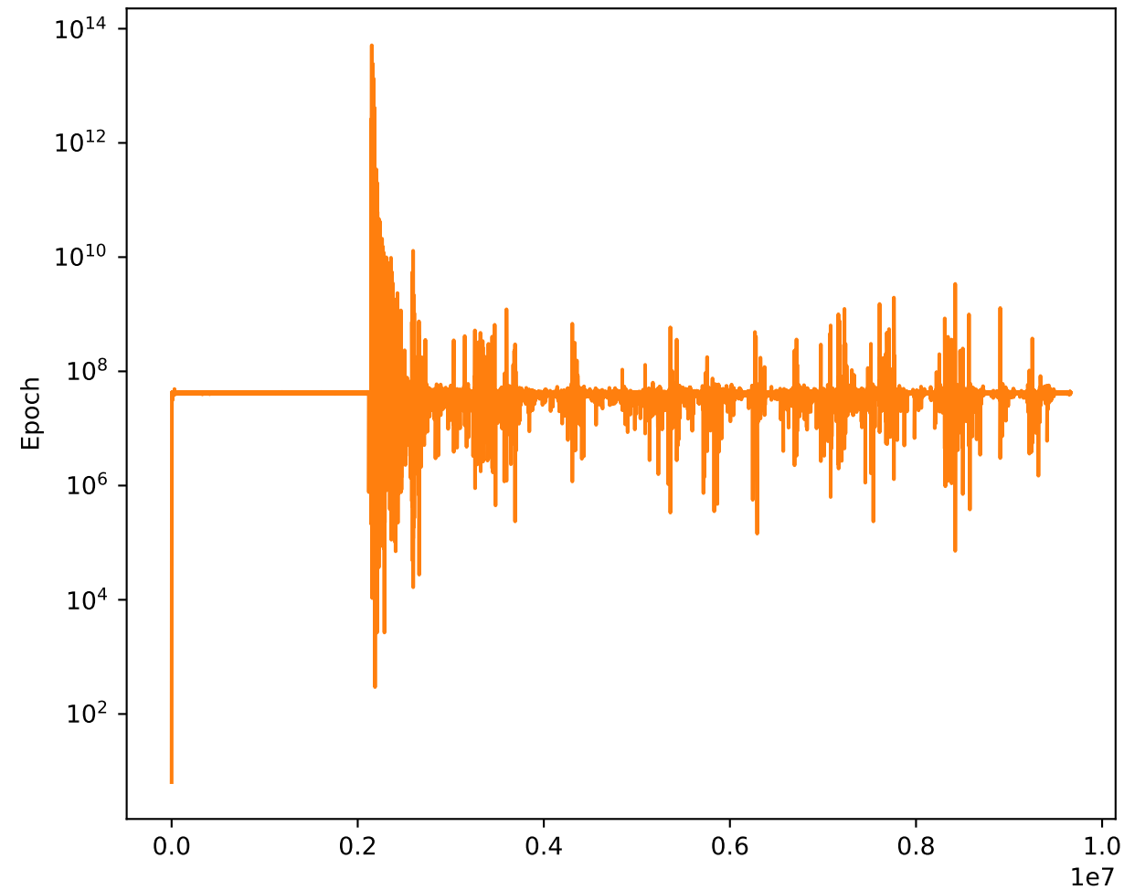
Critic Loss
