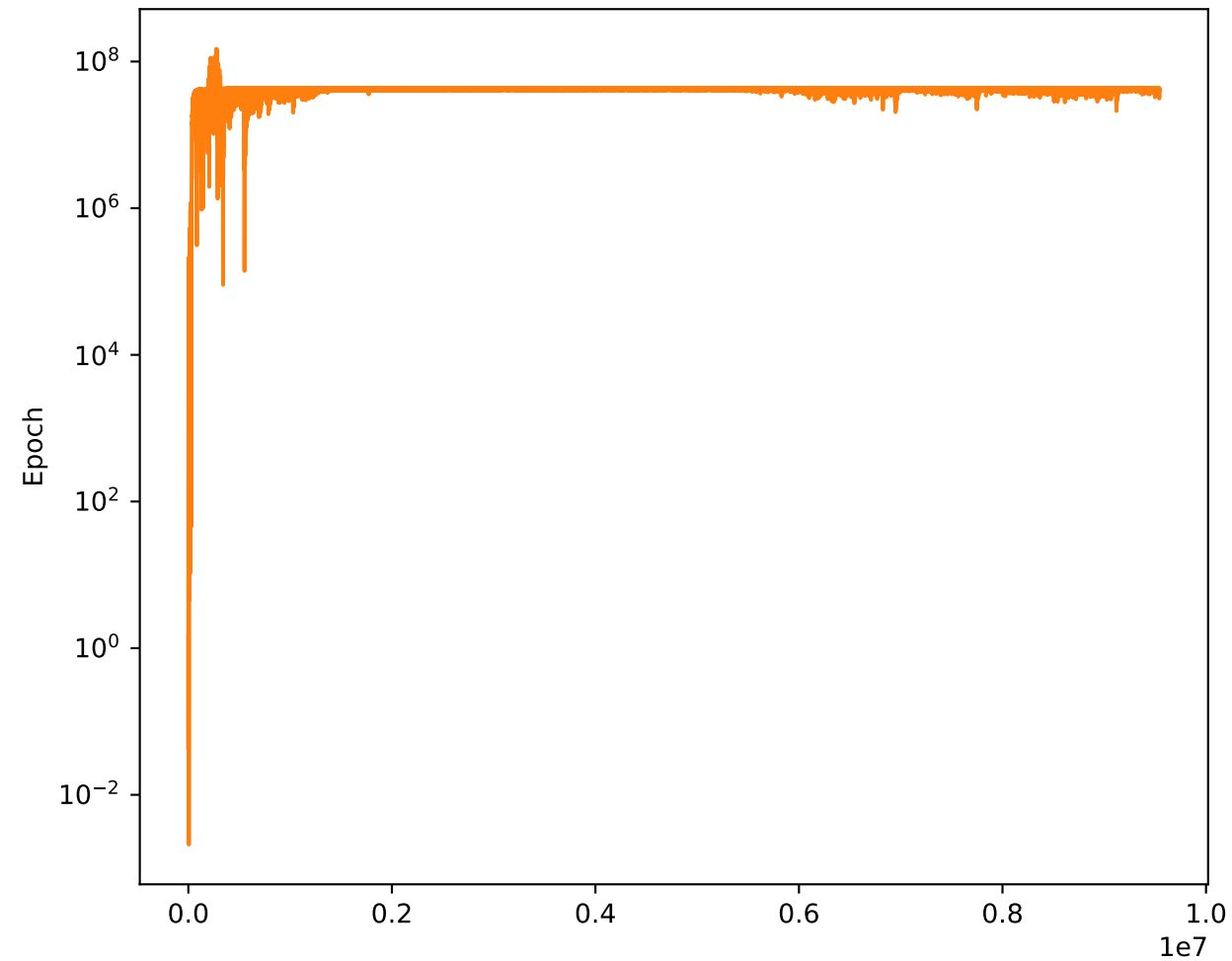
Critic Loss
