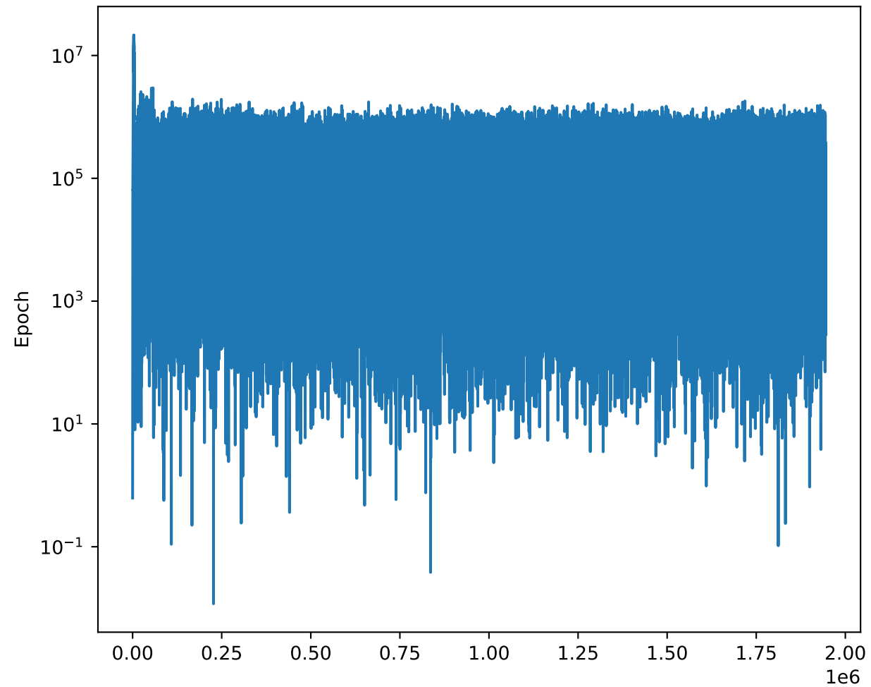
Generator Loss
