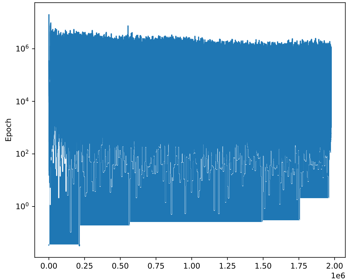
Generator Loss
