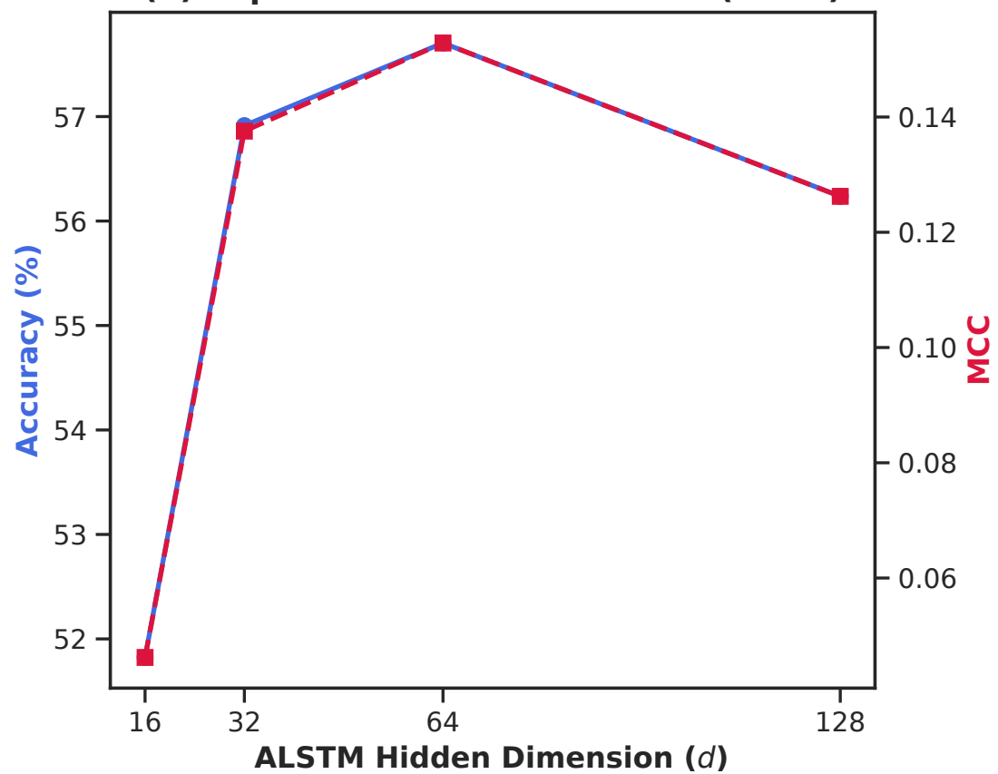
(b) Impact of Hidden Dimension (acl18)
