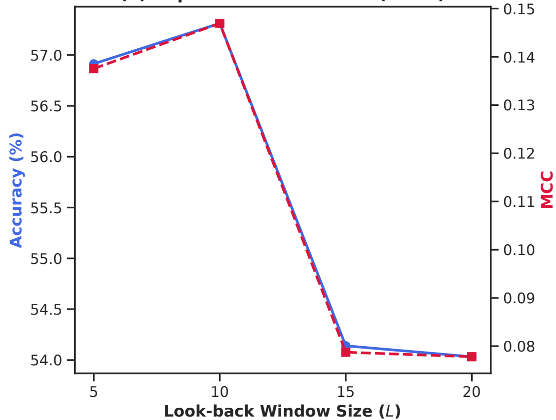
(a) Impact of Window Size (acl18)
