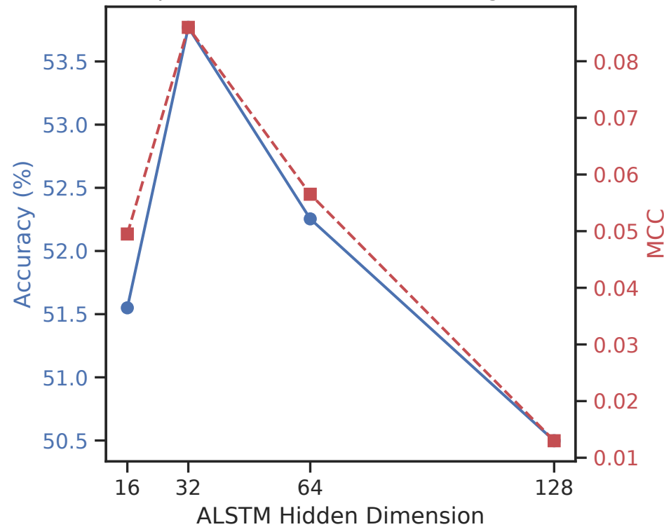
(b) Impact of Hidden Dimension (BigData22)
