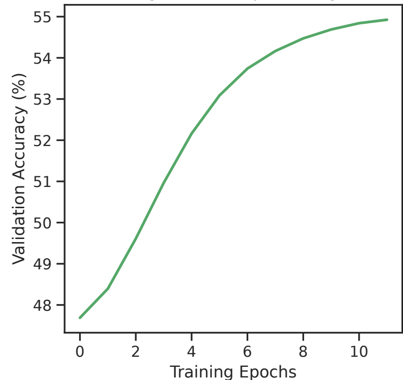
(c) Convergence over Epochs (BigData22)
