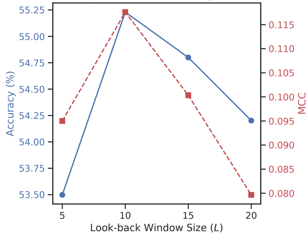
(a) Impact of Window Size (BigData22)
