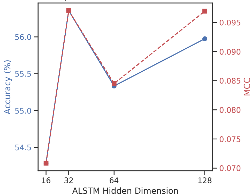
(b) Impact of Hidden Dimension (cikm18)
