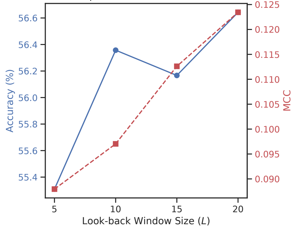
(a) Impact of Window Size (cikm18)
