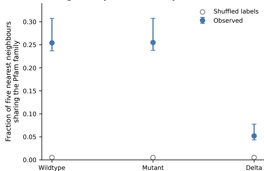
B Local geometry contains family structure
