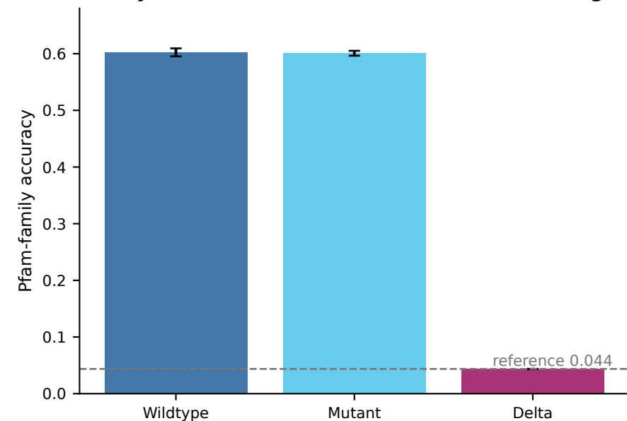
A Family can be decoded from absolute embeddings
