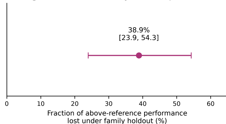
D Leakage fraction with family-bootstrap interval
