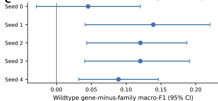
C Gene-held-out performance was higher in every seed
