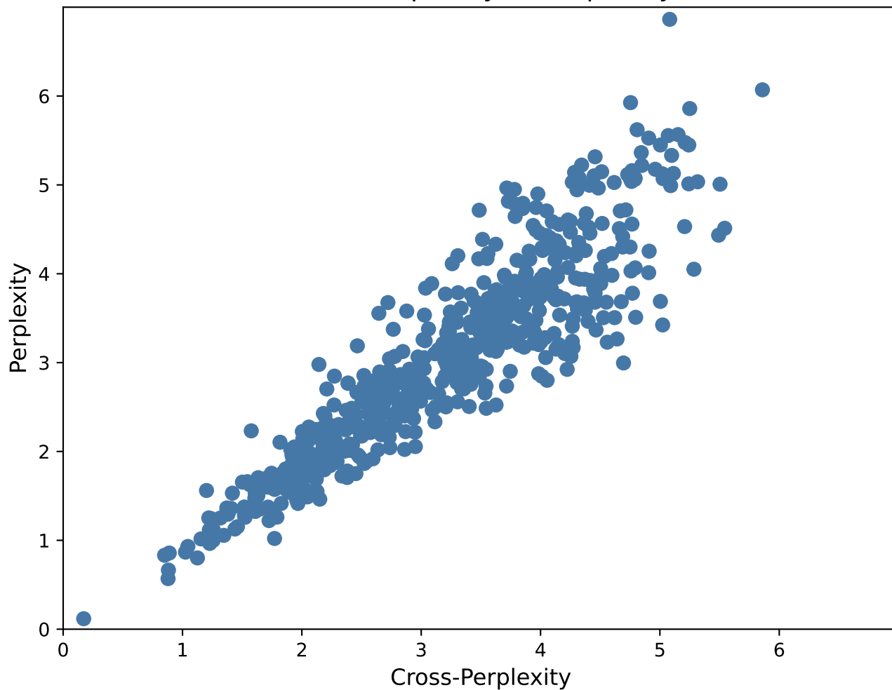
Cross-Perplexity vs Perplexity
