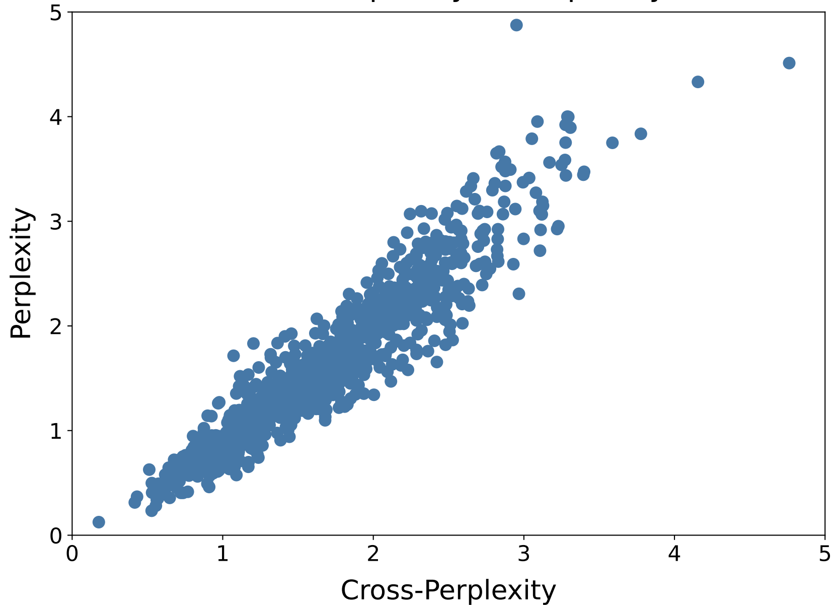
Cross-Perplexity vs Perplexity
