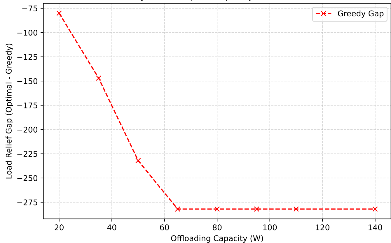
Greedy Value Gap vs Capacity - Workload C1
