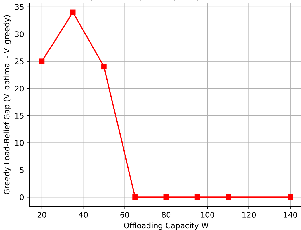
Greedy Value Gap vs Capacity (Workload C1)
