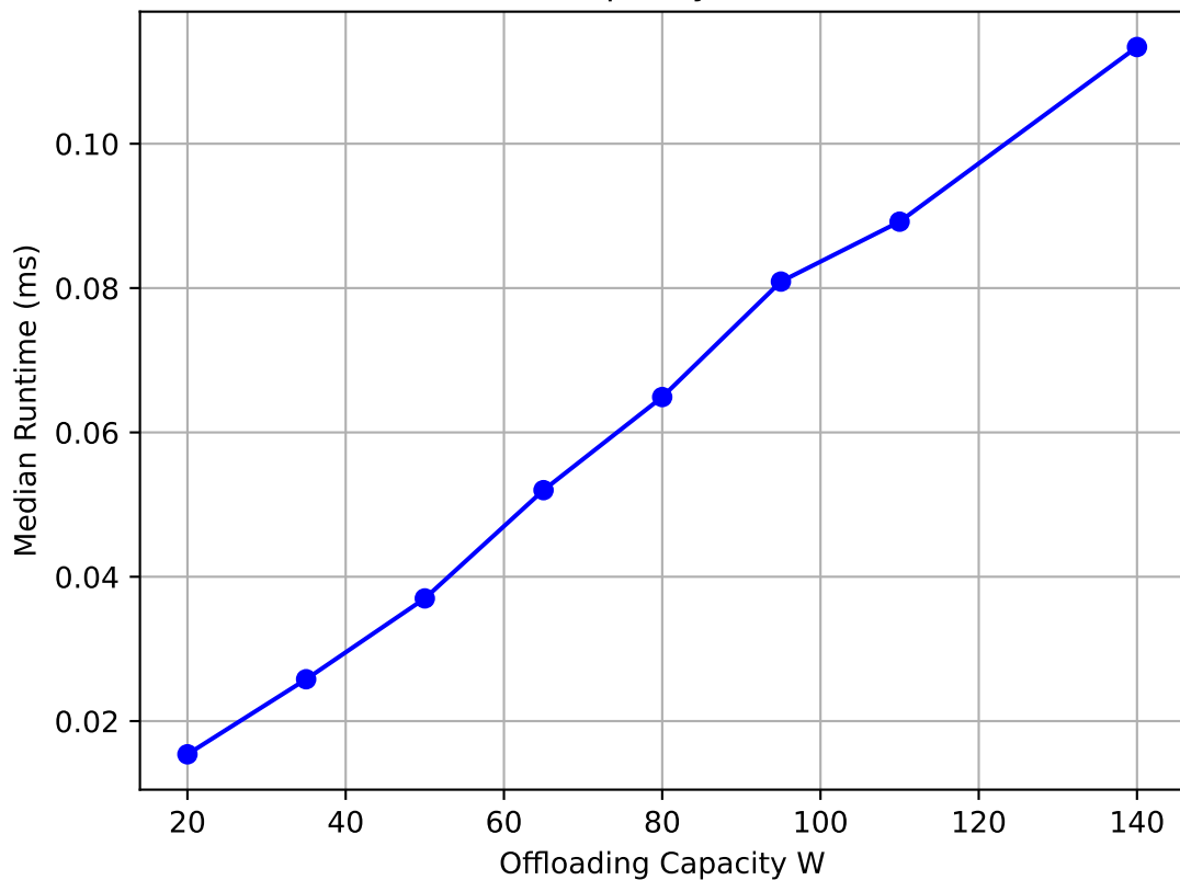
Runtime vs Capacity (Workload C1)
