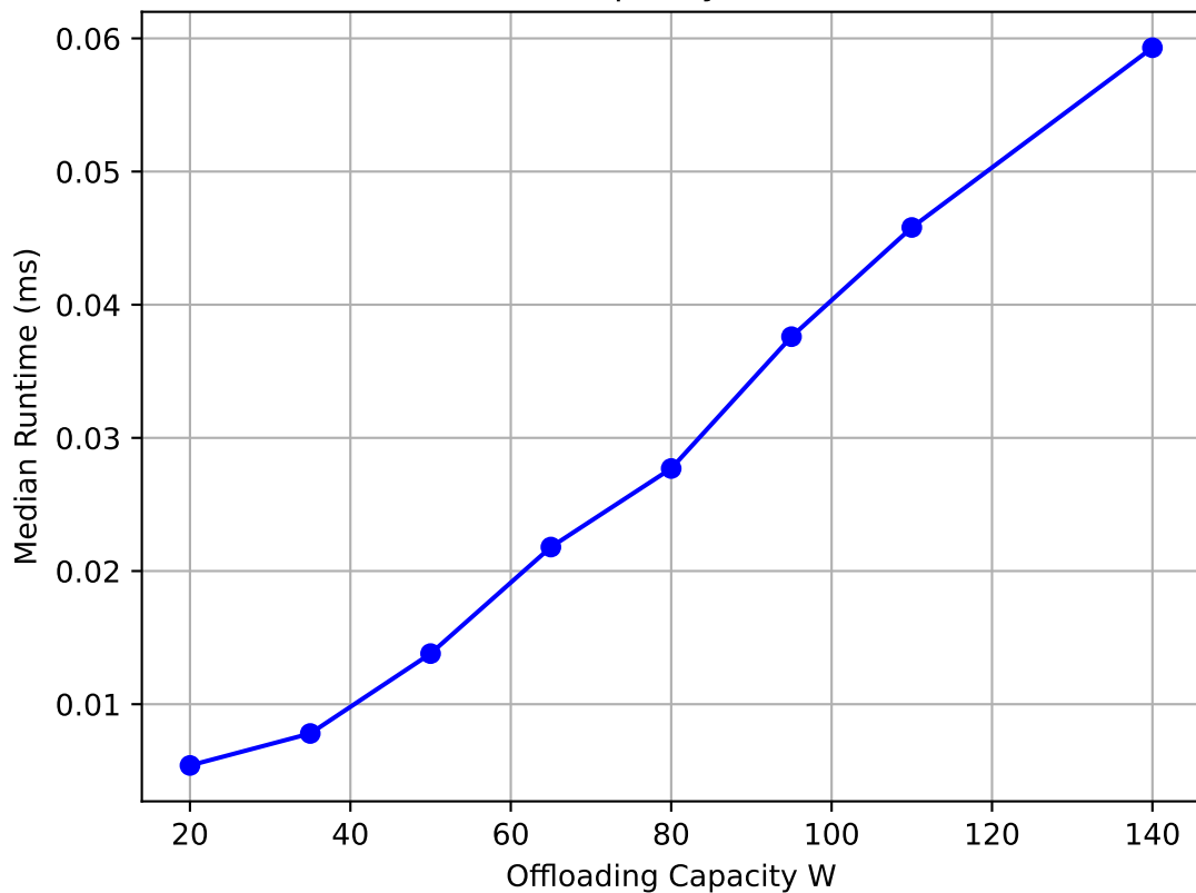
Runtime vs Capacity (Workload C2)
