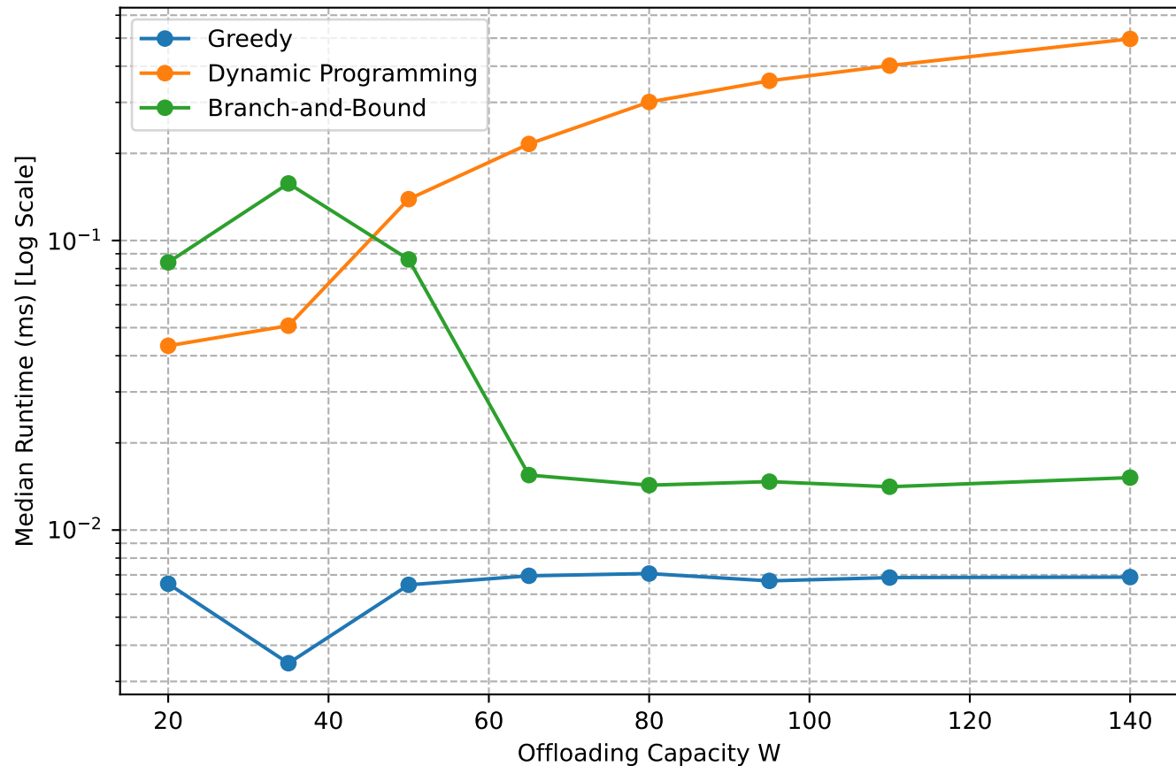
Runtime vs Capacity (C1)
