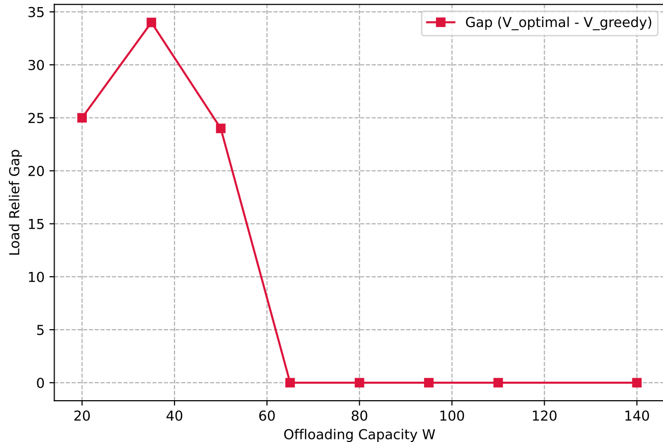
Greedy Value Gap vs Capacity (C1)
