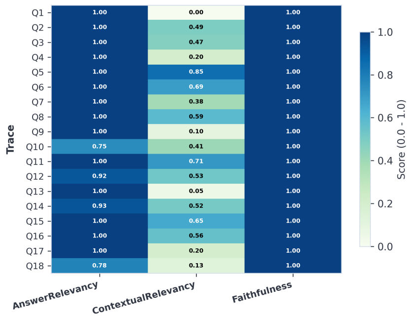
Performance Heatmap
