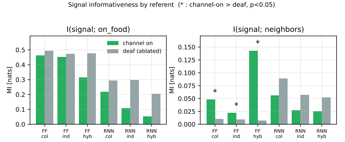
Fig. 4. Visualisation of Table I. Left : information about own food-state is as high or higher when deaf — it is “free”. Right : information about the configuration of groupmates exceeds the deaf baseline only for the feedforward agents (*: on>deaf, p < 0.05 ), and most strongly under the hybrid — the signature of real, function-bearing communication.
