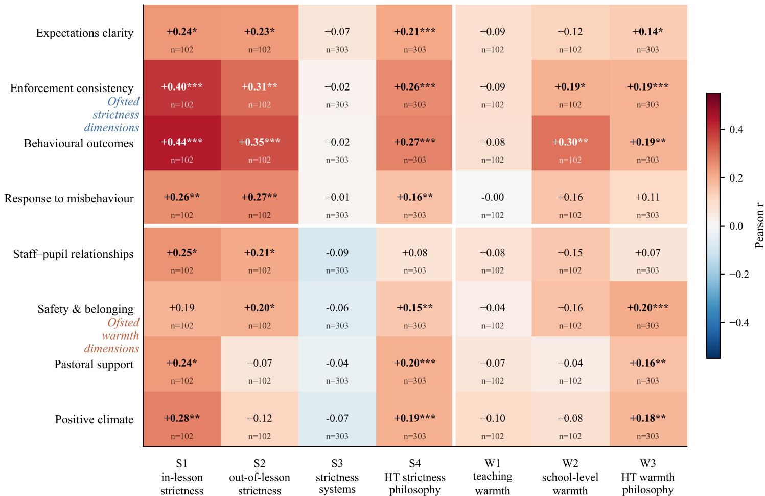
Figure C — Sub-score correlation matrix Ofsted LLM sub-dimensions vs interview/visit sub-scores (* p<.05 ** p<.01 *** p<.001)
