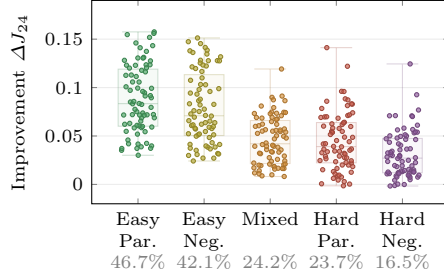
Fig. 3: Per-question CRW improvement \Delta J_{24} on Bern across 75 questions and 5 attack settings (E5-Instruct, \alpha^* = 0.4 ). Gray percentages indicate the mean share of distortion mitigated \overline{\Delta J_{24}}/(1 - \overline{J_{24}}) , with uniform baseline J_{24} = 0.810 across all conditions.
