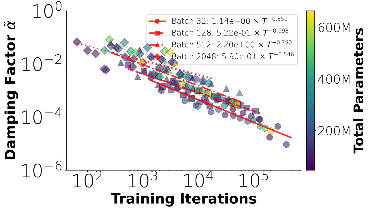
Figure C: Larger Batch Allow Larger Damping Schedule. Same setting as in Figure 5: we use \alpha(t) = \tilde{\alpha} \times (1 + t) and sweep \tilde{\alpha} across model size and iterations. Increasing batch size allows for larger constant \tilde{\alpha} .
