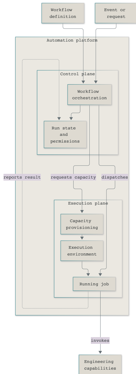
Figure 2. Logical platform responsibilities. Provisioning can contain control logic of its own, while the execution environment supplies the resources and authority available to a running job.
