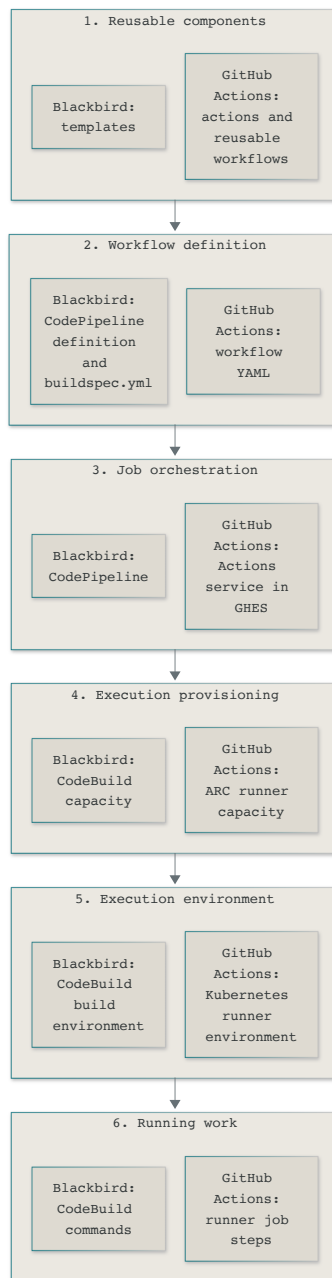
Figure 3. Each numbered stage contains the corresponding Blackbird and GitHub Actions components. The downward arrows show the progression from reusable material to running work; either implementation may invoke build, scan, artifact and deployment capabilities.
