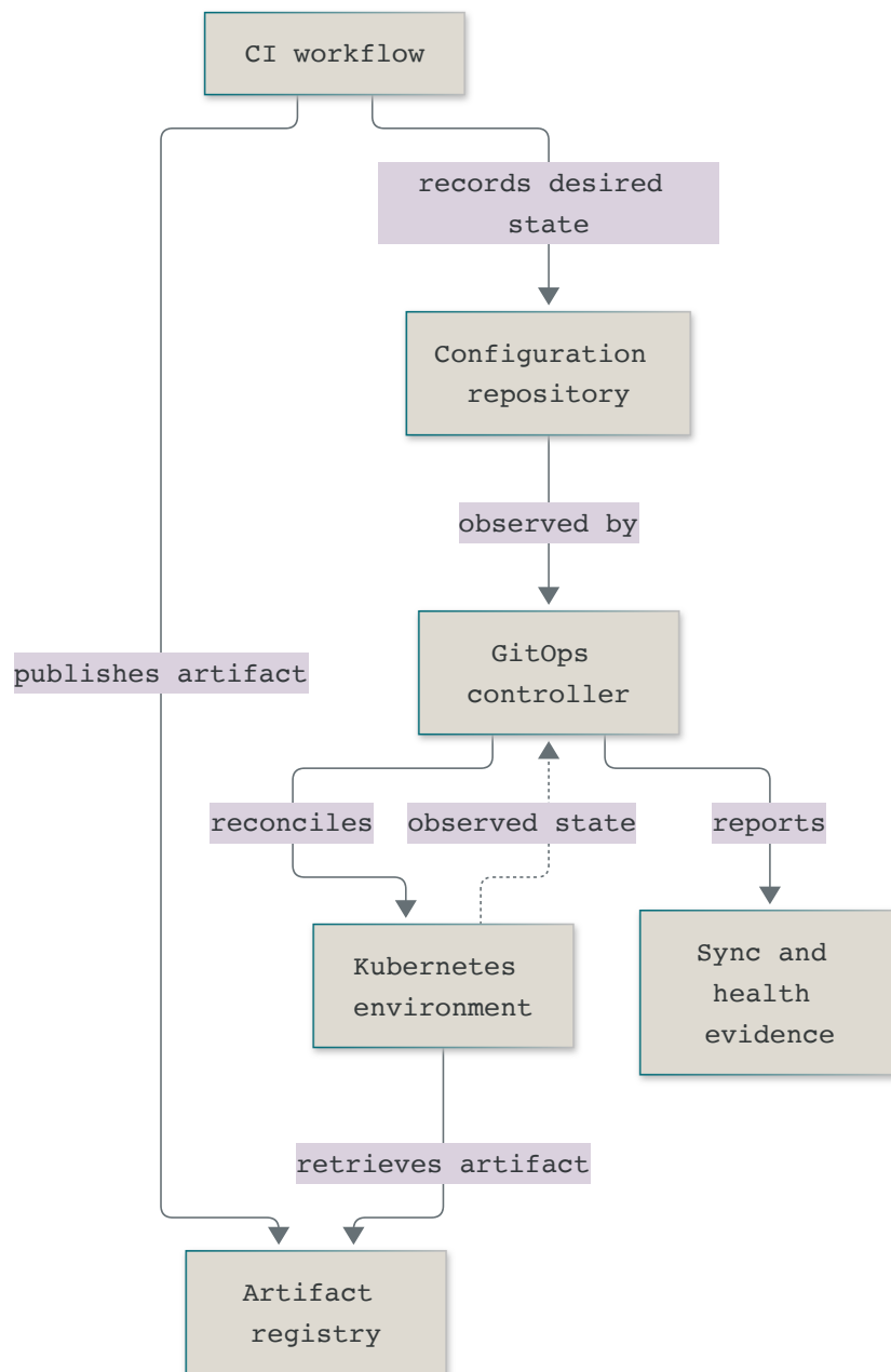
Figure 4. A representative Git-sourced Kubernetes delivery path. Artifact publication and a change to desired state can finish before the controller reconciles the environment and reports the observed result. Flux can also consume desired state from an OCI registry.
