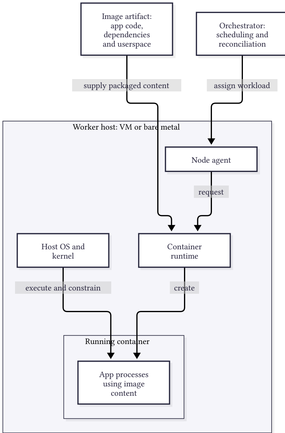
Figure 1 places the packaged software, the orchestration system and the execution host in relation to one another.
