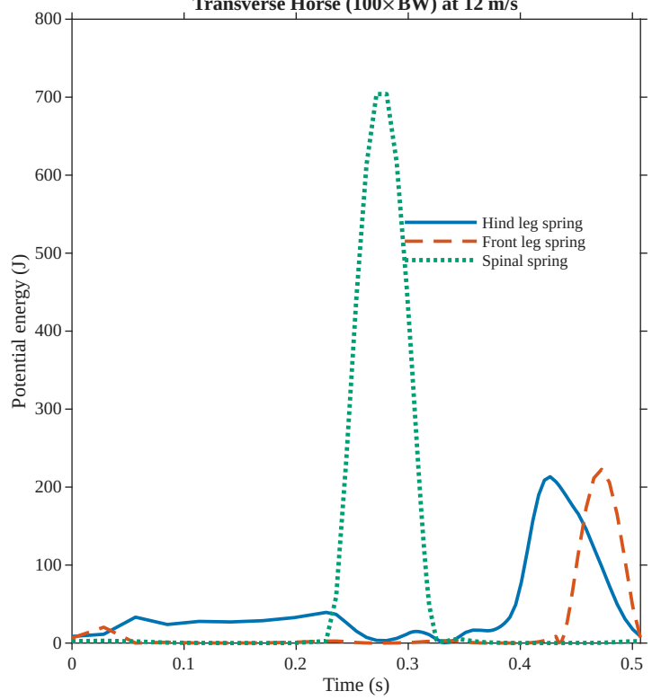
Transverse Horse ( 100\times BW ) at 12 m/s
