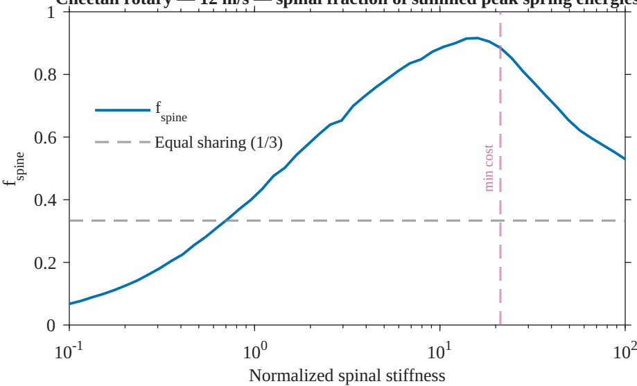
Cheetah rotary — 12 m/s — spinal fraction of summed peak spring energies
