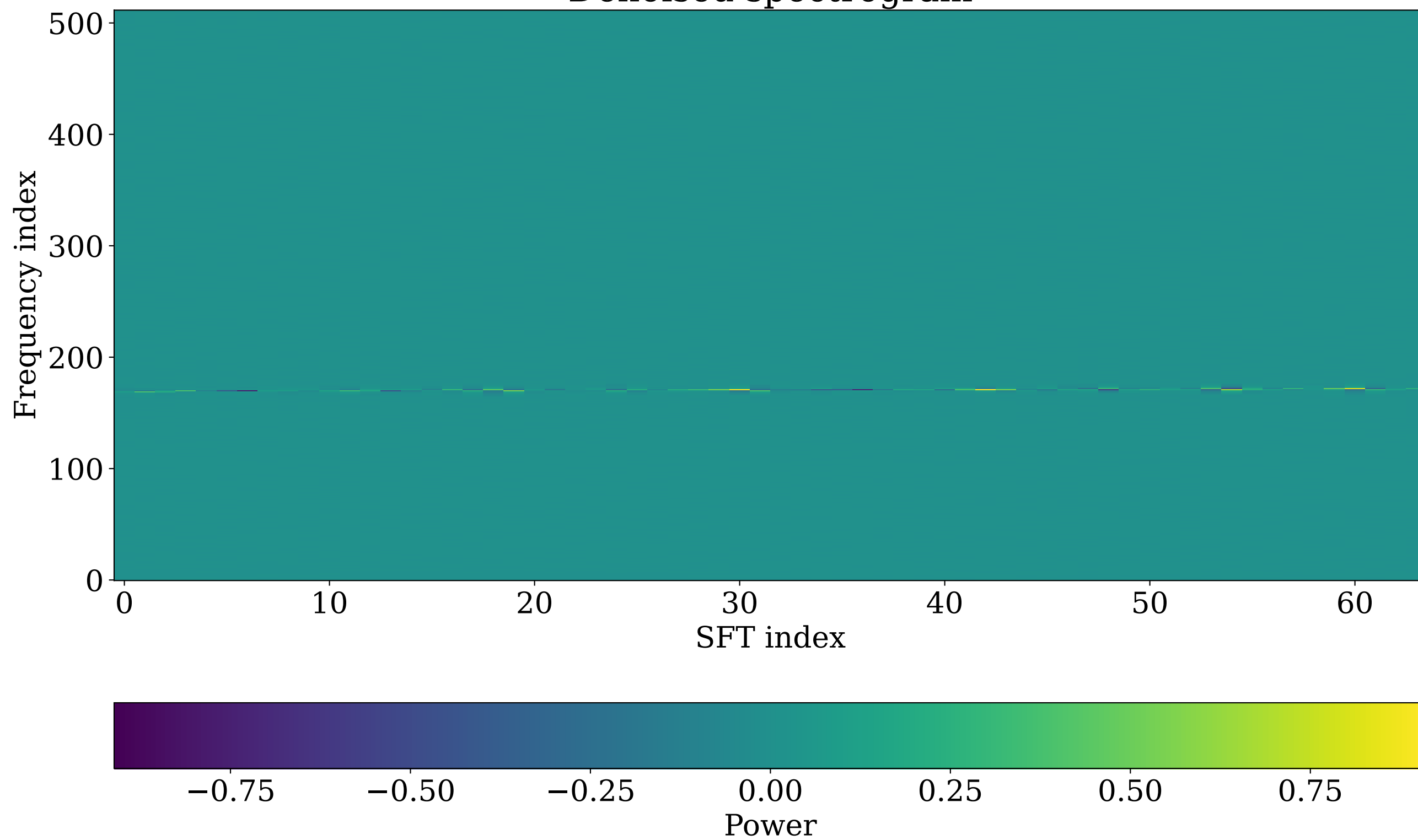
Denoised spectrogram
