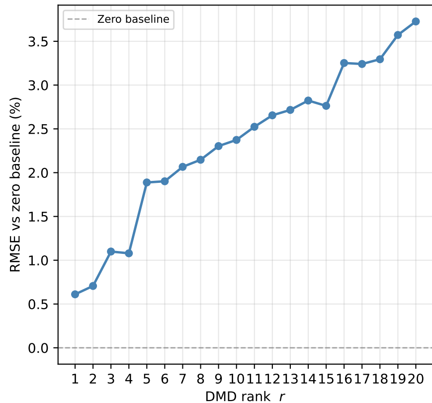
Prediction error
