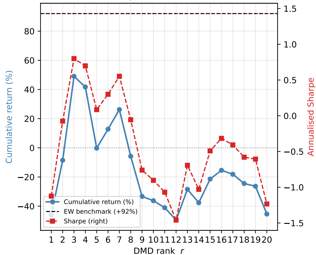
Portfolio performance vs rank
