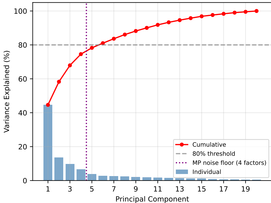
(a) Scree Plot with Random-Matrix Noise Floor
