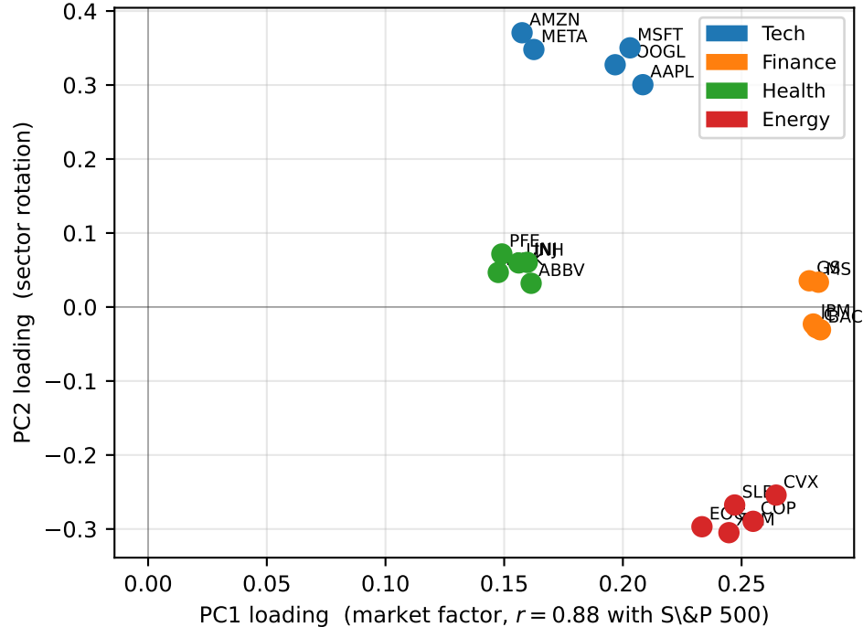
(b) Stock Loadings on First Two PCs
