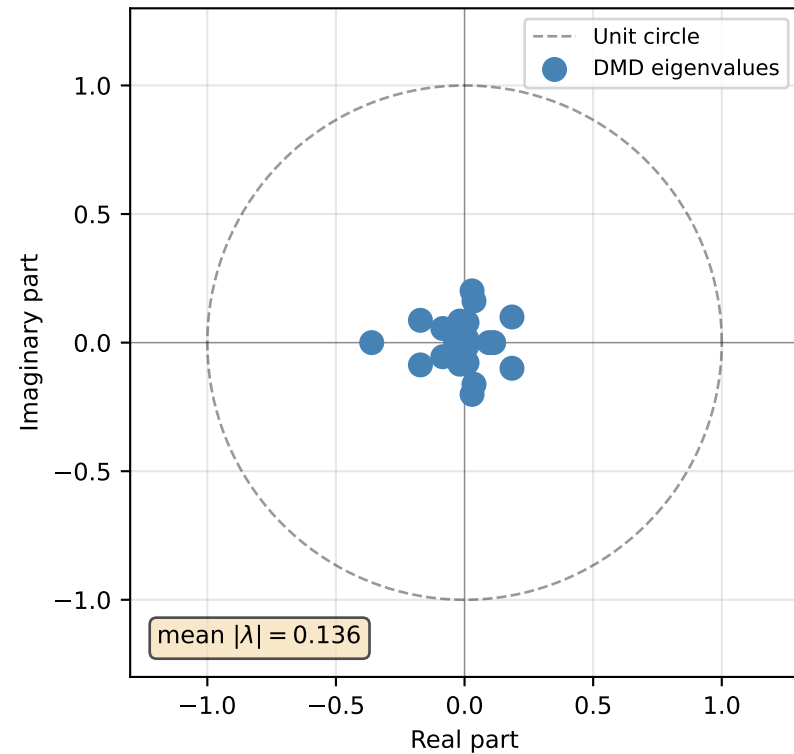
(a) DMD Eigenvalue Spectrum (trained on 2020–2022 returns)
