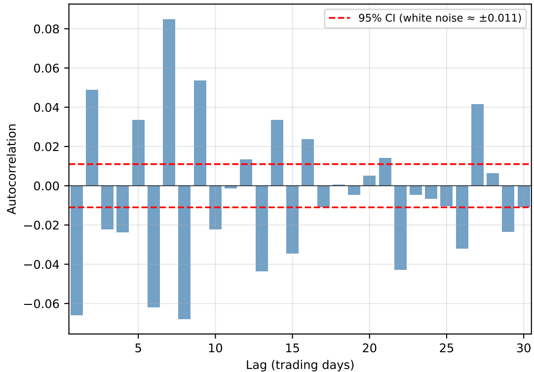
(b) Autocorrelation of Daily Returns (all 20 stocks pooled)
