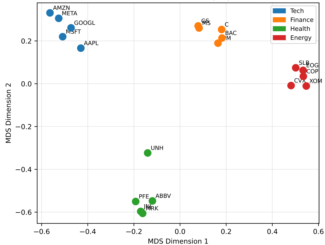
(a) Classical MDS Embedding ( d_{ij} = \sqrt{2(1 - r_{ij})} )
