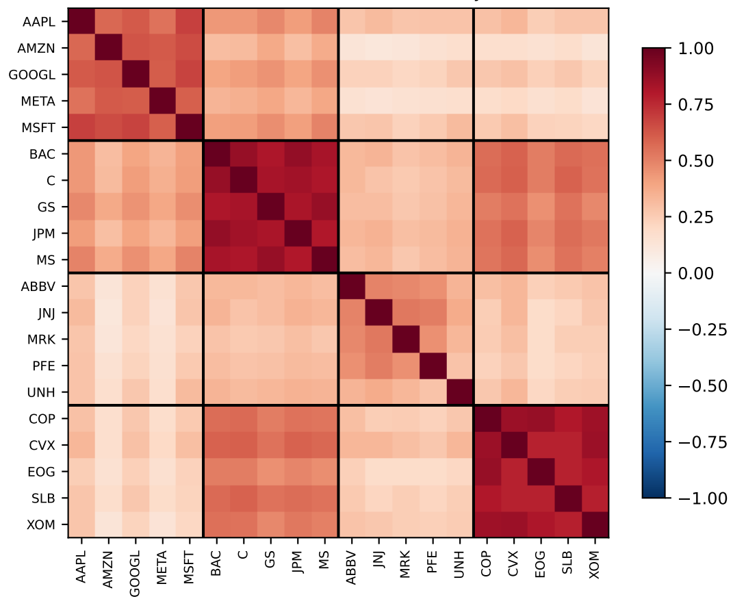
(b) Return Correlation Matrix (Sorted by Sector)
