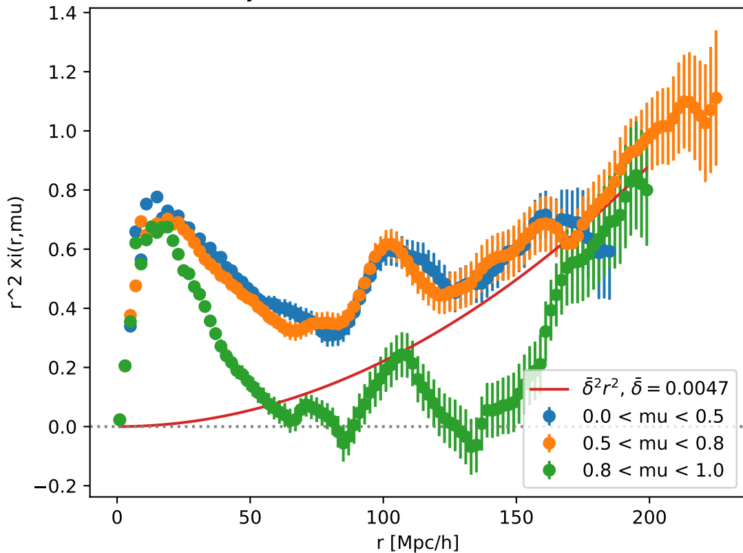
density correlation function (130k skewers)
