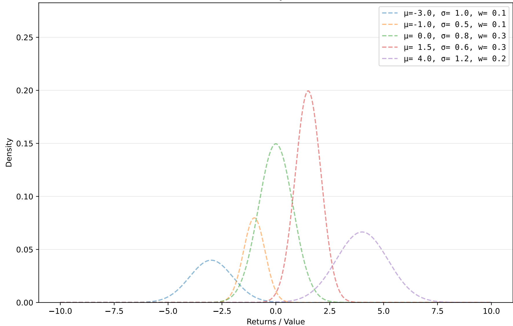
Mixture Normal Density with VaR & ES (5%)
