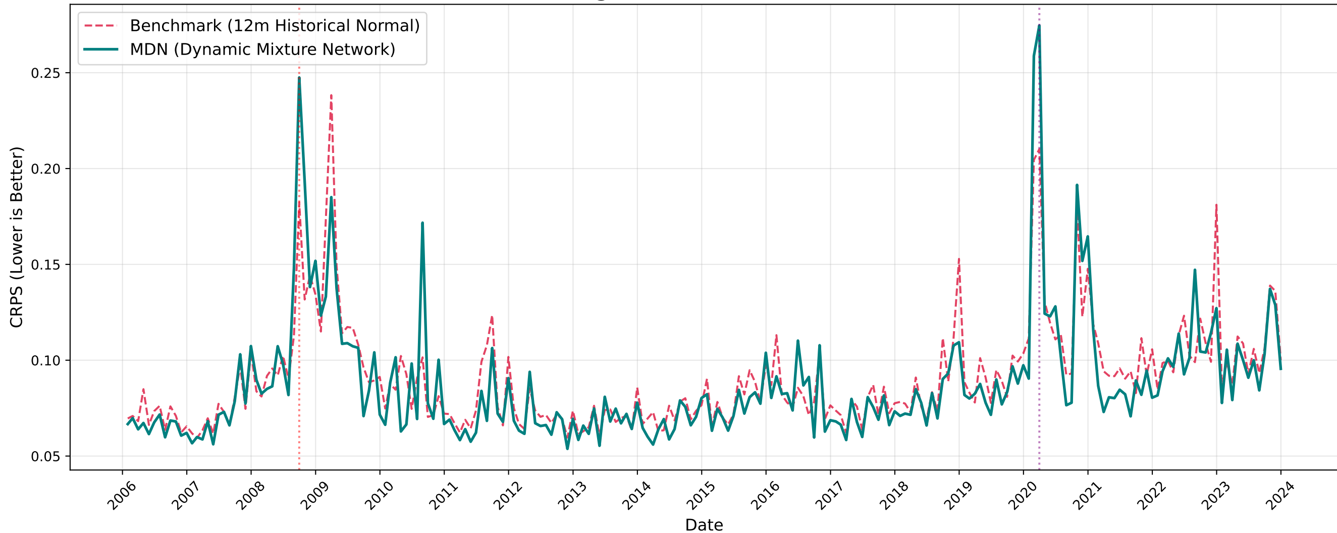
Cross-Sectional Average CRPS: MDN vs. Traditional Benchmark
