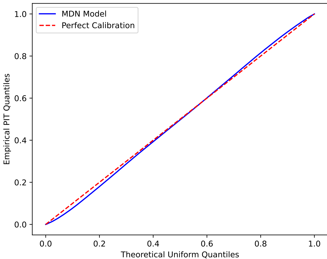
PIT QQ-Plot
