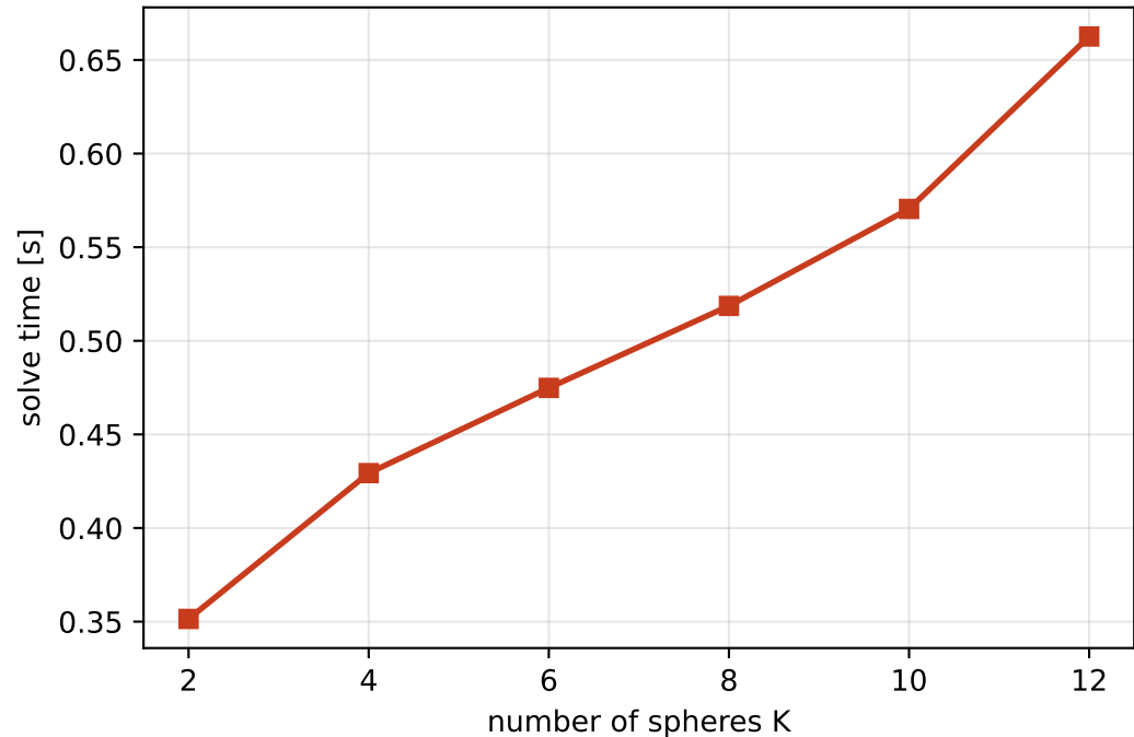
Runtime vs number of objects
