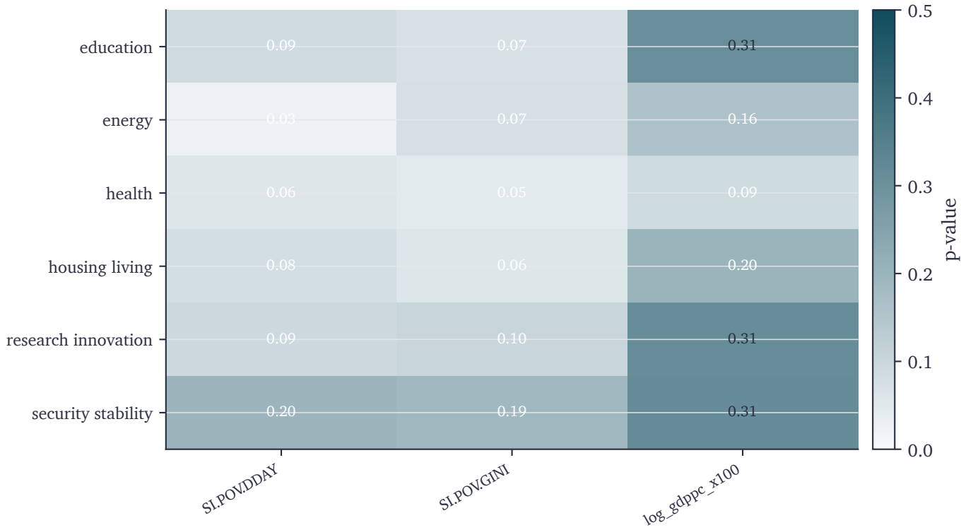
Dumitrescu-Hurlin panel Granger causality (p-values)
