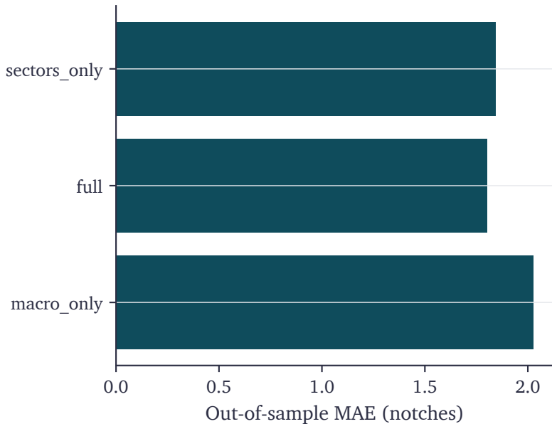
Prediction error
