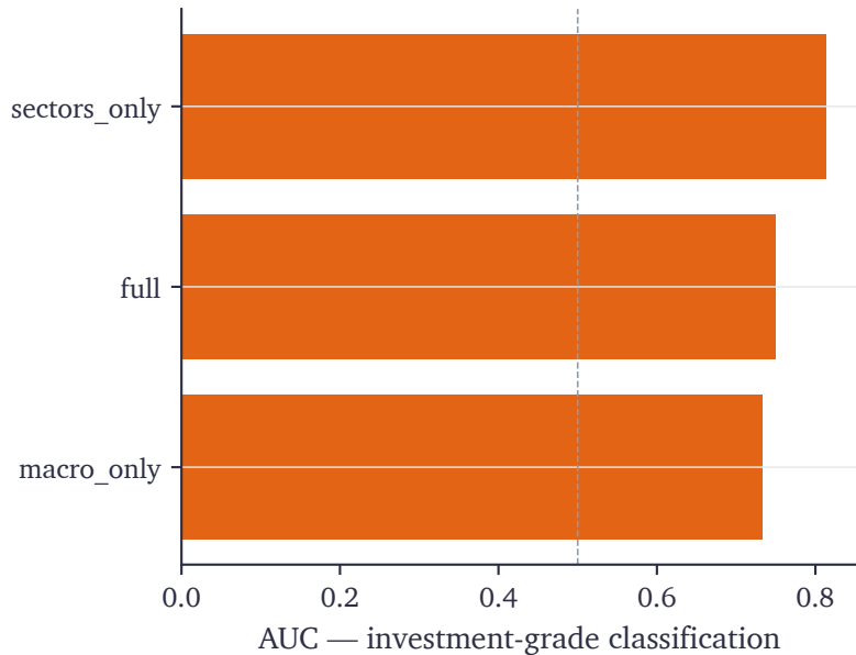
Discrimination
