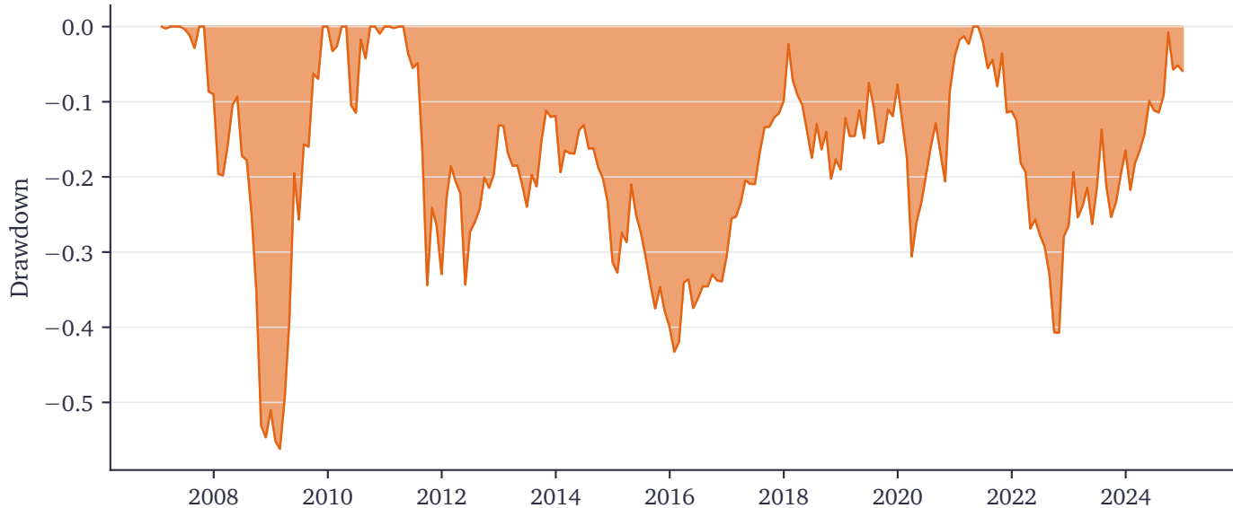
Drawdown — long-only top quintile
