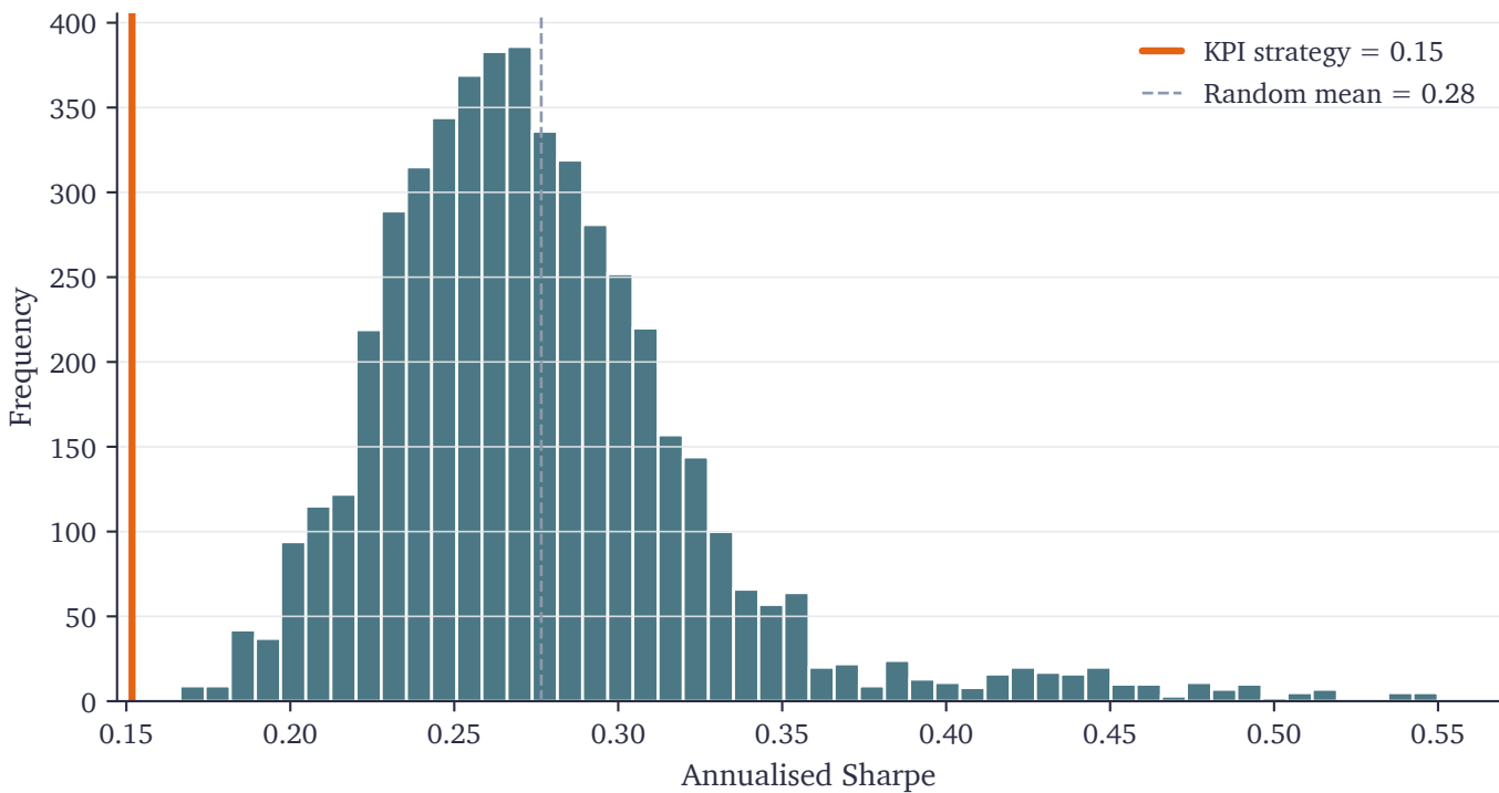
Stationary-bootstrap distribution of Sharpe ratios — 5 000 random 4-country baskets
