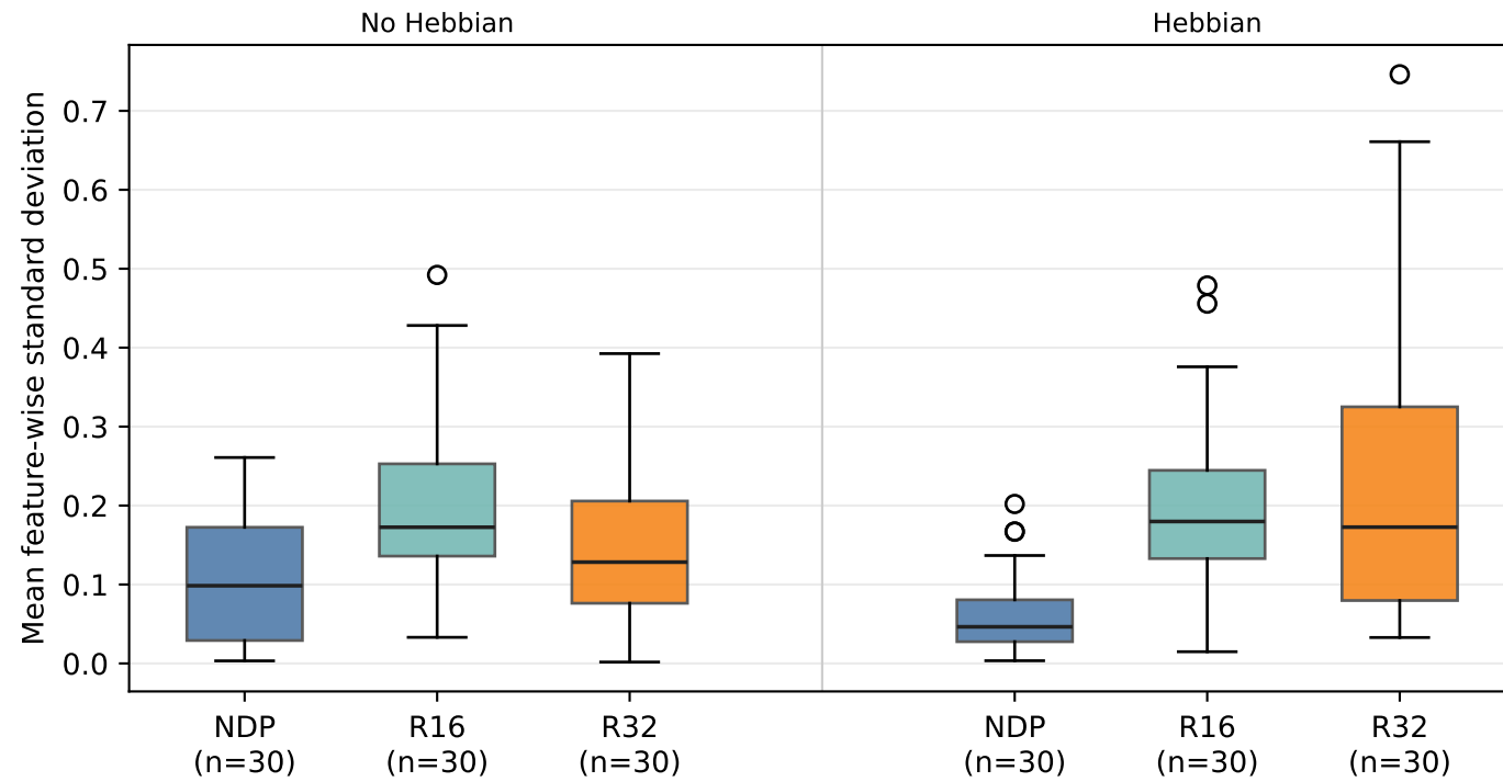
Acrobot
