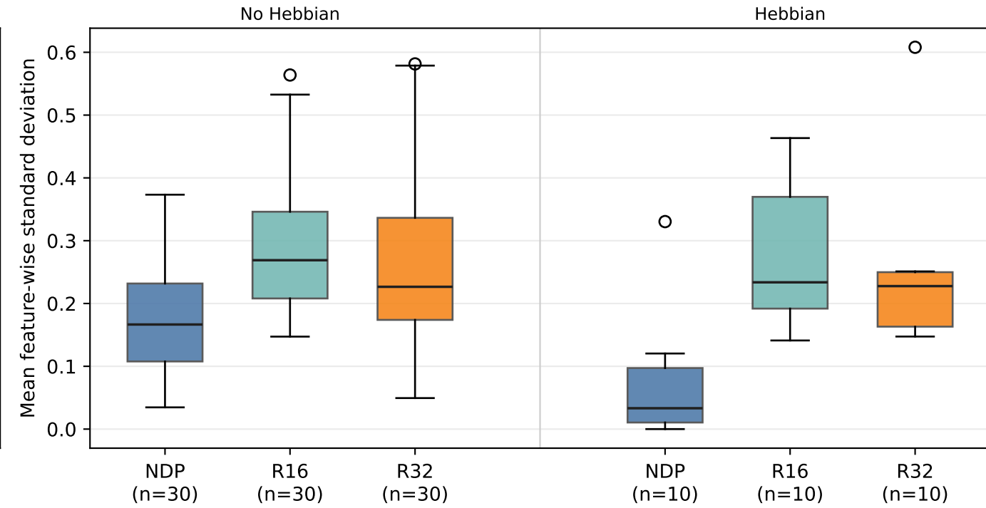
MountainCar
