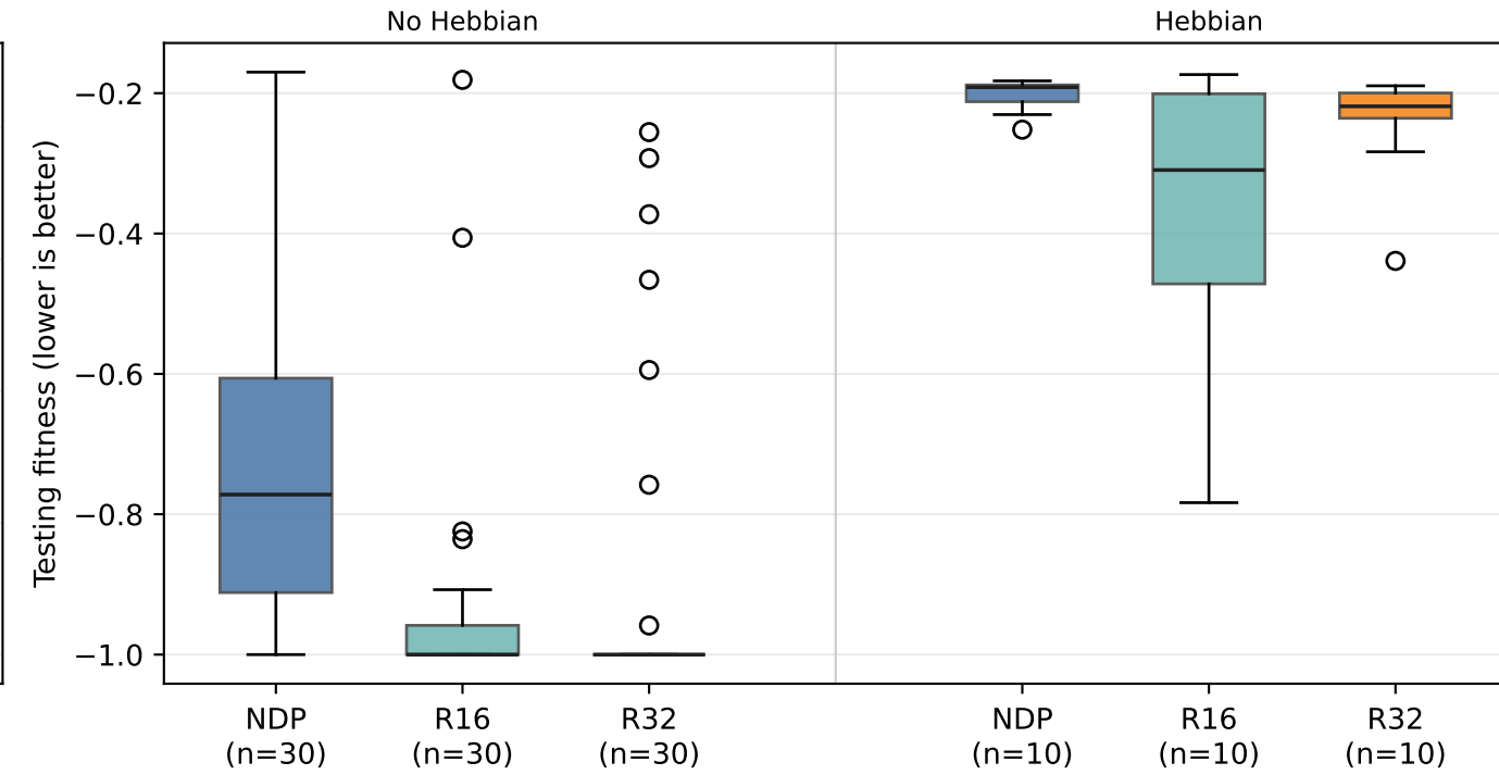
MountainCar
