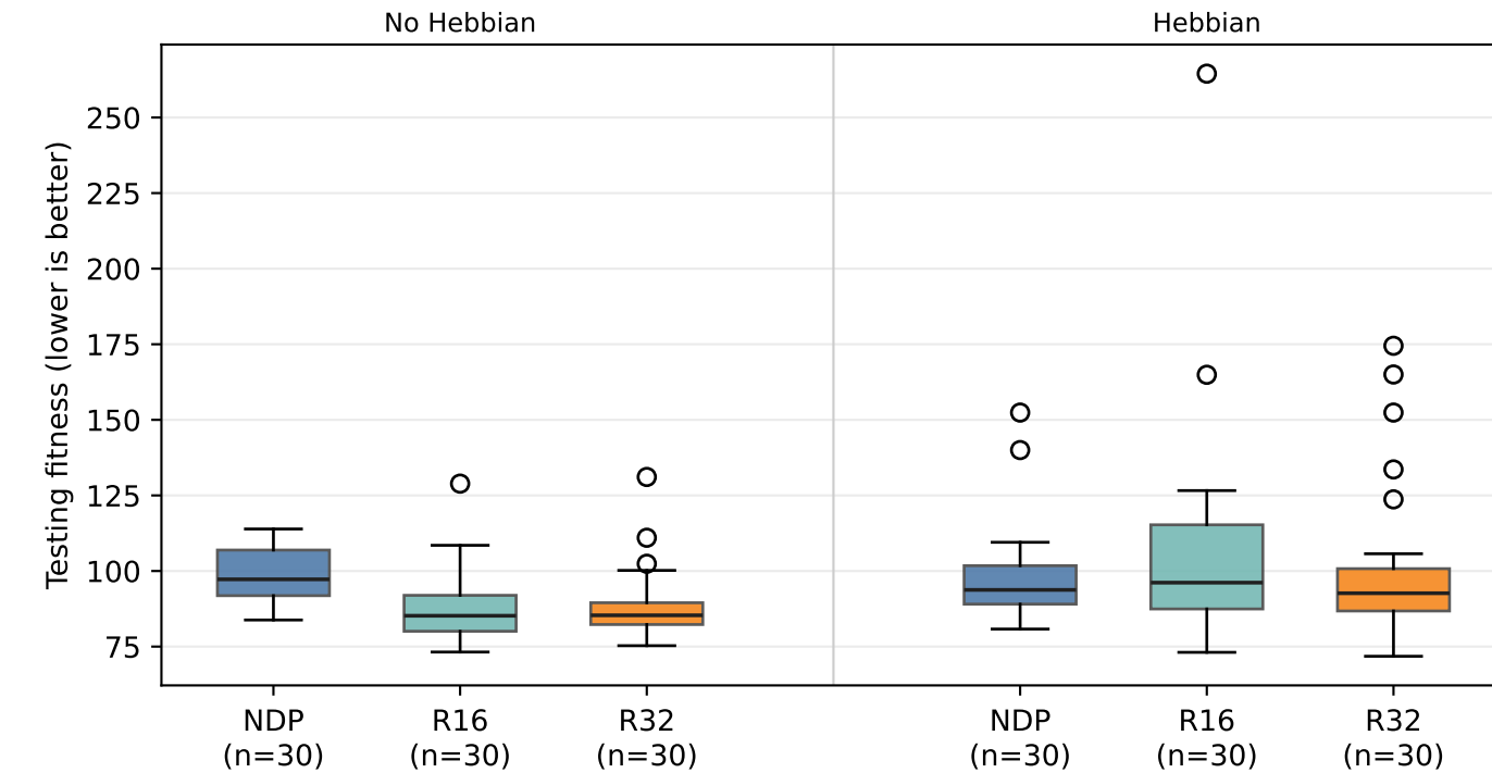
Acrobot
