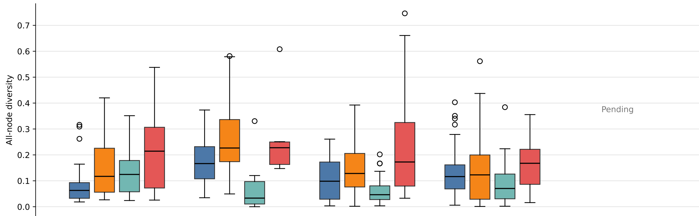
Node-state diversity: NDP vs R-NDP 32
