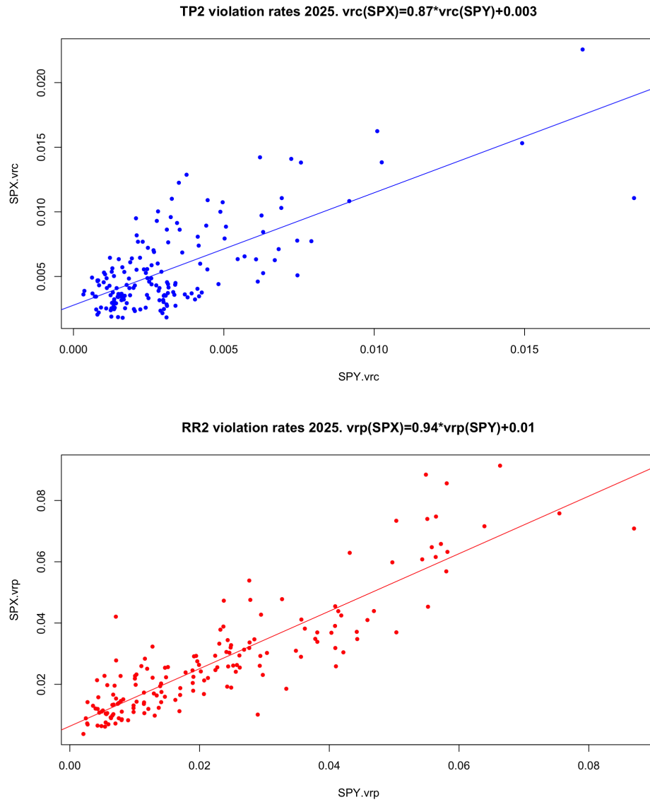
Figure 2: Scatter plots for the daily violation rates for SPX and SPY, which show the correlation among them.
