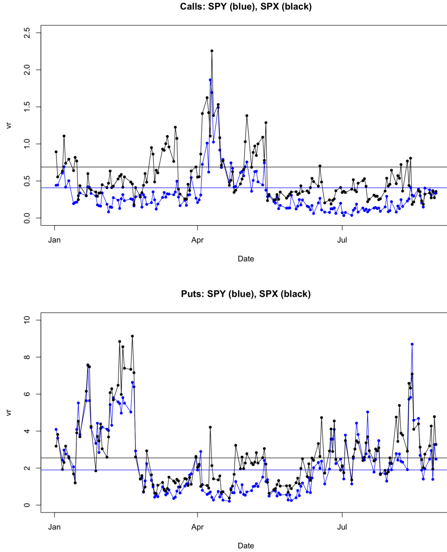
Figure 1: The violation rates for TP2/RR2 violations for each day in the 2025 dataset, comparing SPY and SPX. The horizontal lines show the average violation rates from Table 1.
