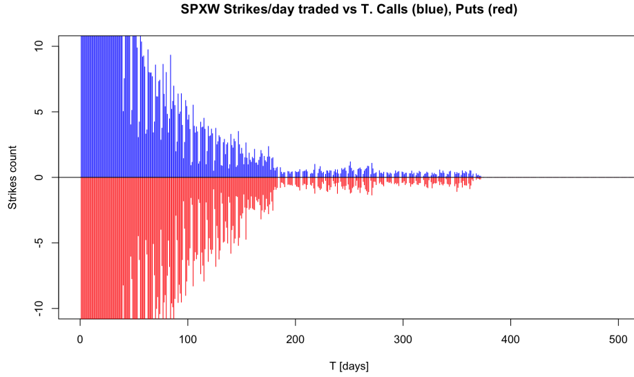
Figure 2: The number of strikes traded for SPXW options vs maturity T , separately for calls and puts. This uses the first 100 days of 2025.
