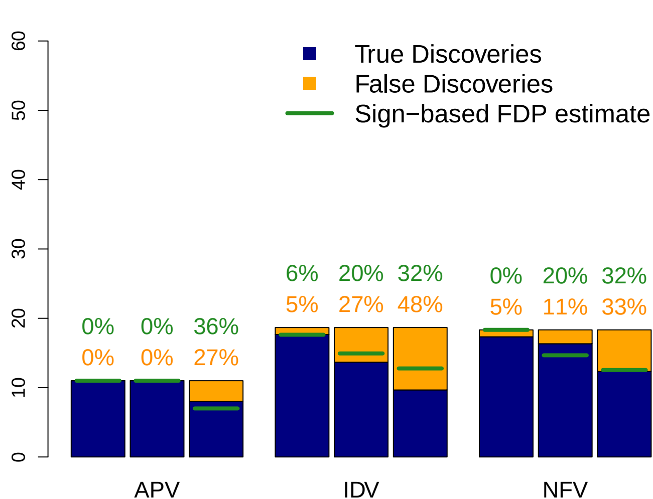
Local FDP by thirds
