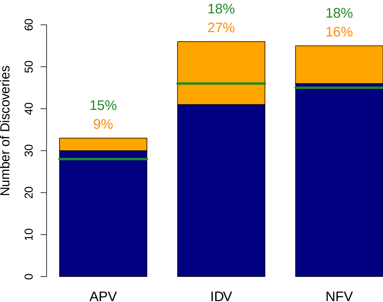
Knockoffs aggregate (tail) analysis
