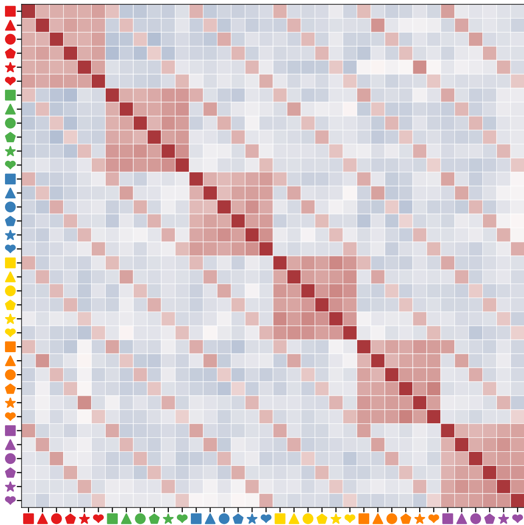
Gemma 3 12B - Avg Probe-Based (PCA) Concept Vectors
