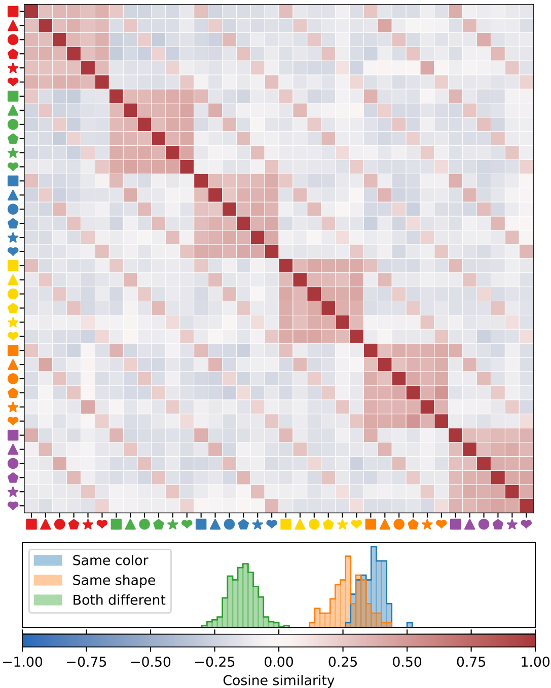
Gemma 3 12B - Avg Probe-Based (Raw) Concept Vectors
