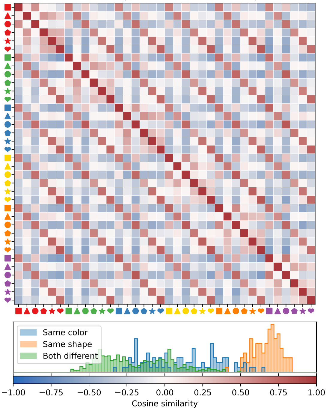
InternVL 2.5 8B - Avg Probe-Based (PCA) Concept Vectors
