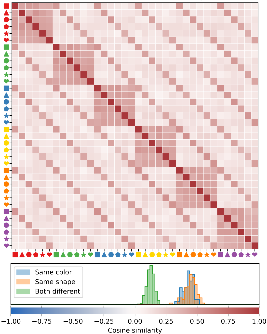
InternVL 2.5 8B - Probe-Based (Raw) Concept Vectors
