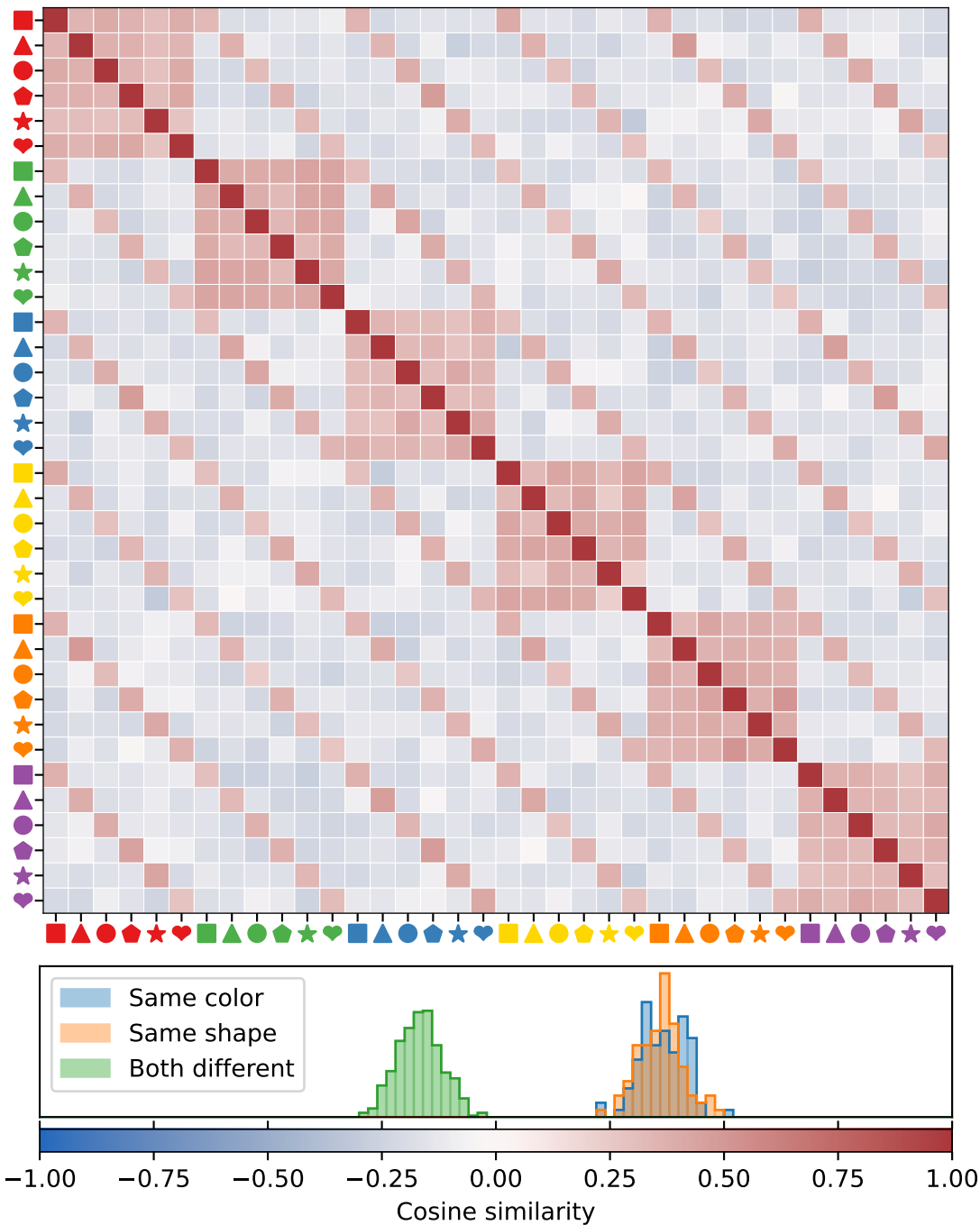
Qwen 2.5 7B - Avg Probe-Based (Raw) Concept Vectors
